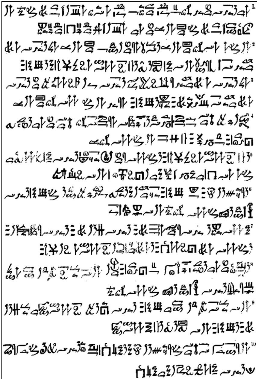
Fig. (3) Hieratic Text of the First Part of the D'Orbiney Papyrus EA.10183. [46]
