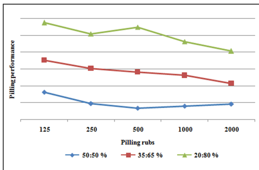
Fig. (3): The effect of three cotton/polyester blend ratios on pilling phenomenon of their woven fabrics under five rubbing cycles.
